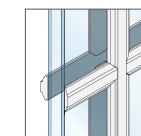
COLOR-MATCHED SIMULATED-DIVIDED-LIGHT CONTOUR 7/8"
